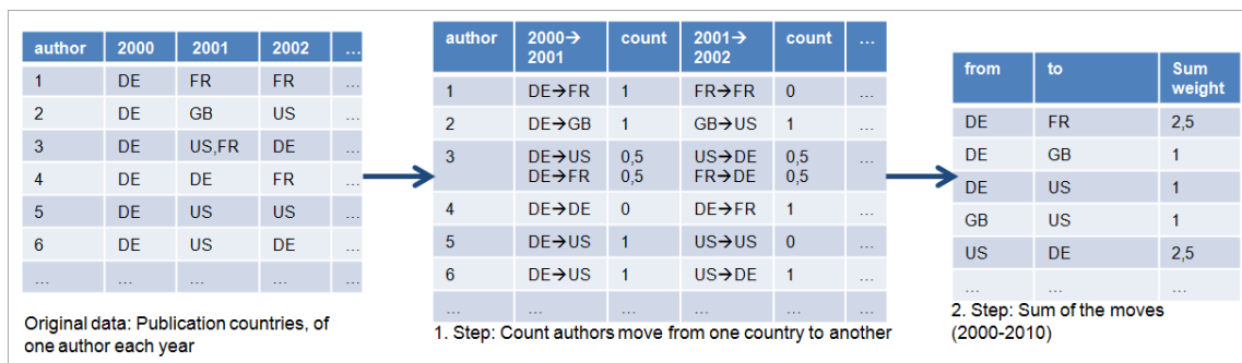
Figure 2: Data processing for tracking scientific mobility from one country to another
