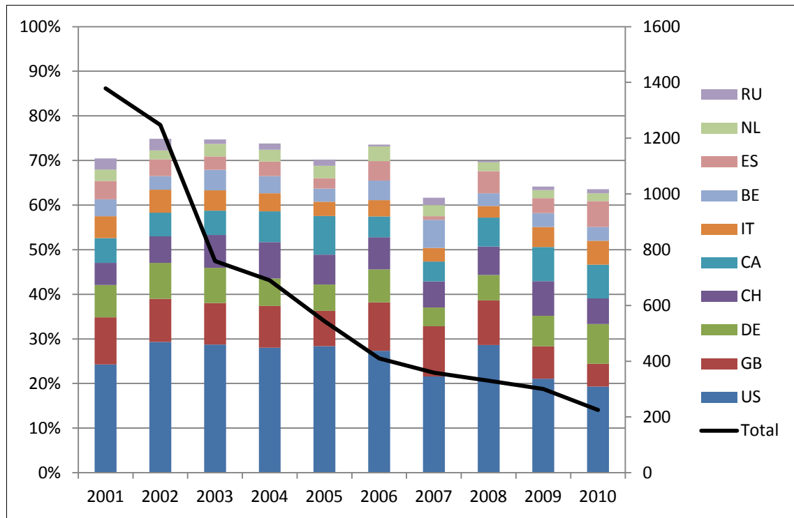
Figure A-7: Top 10 countries to which French scientists move.
