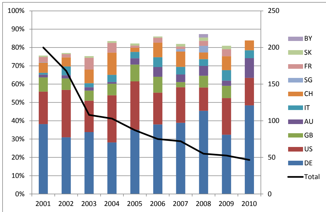
Figure A-3: Top 10 countries to which Austrian scientists move.
