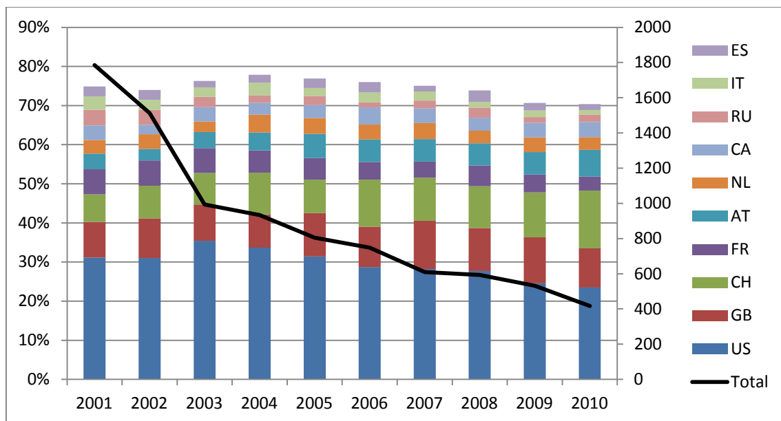
Figure 14: Top 10 migration countries for separate years.
